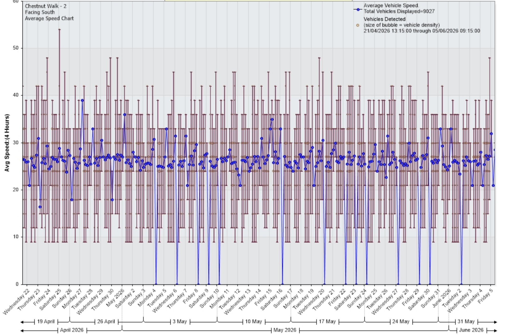
Average Vehicle Speed (MPH) vs. Time [Chestnut Walk - 2:Incoming]
