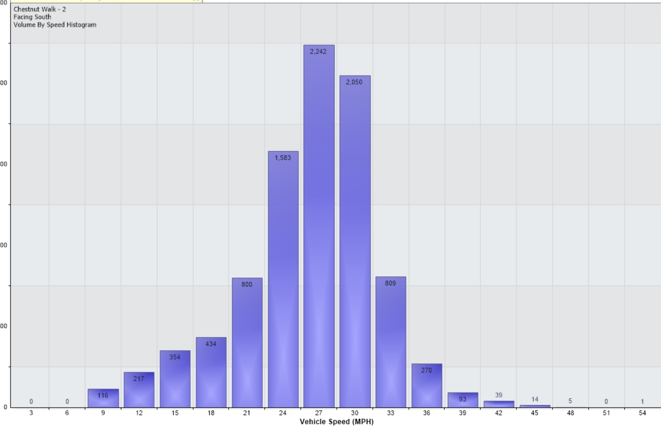
Vehicle Counts Vs. Speed [Chestnut Walk - 2: Incoming]
